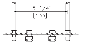
Optional suspension bracket available for 5-1/4" [133] spacing.
